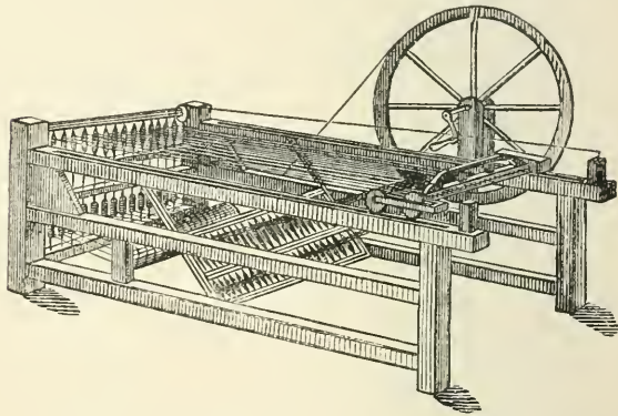
HARGREAVE'S SPINNING-JENNY.
